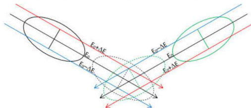
FIG. 3. Crossing angle collision with opposite dispersion.
