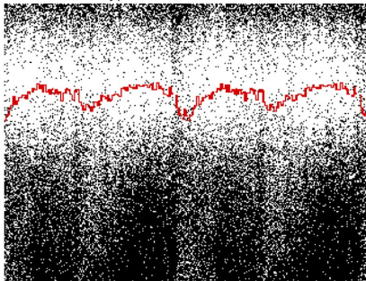
EA/EBtype (0.61) EW type (0.19), Unknown (0.15)
