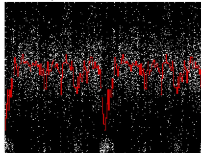
EA/EBtype (0.46) Junk (0.22), Unknown (0.19)
