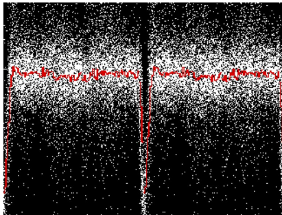
EA/EBtype (0.62) Unknown (0.15), EW type (0.14)
