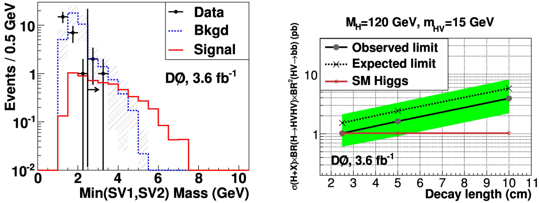
Figure 5: The smallest secondary vertex mass in the event (left), and limits on the SM Higgs boson production cross section, for a \nu -hadron mass of 15 \text{GeV}/c^2 (right).
