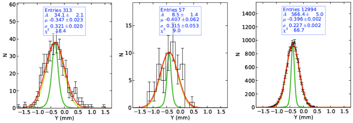
Figure 4: Measured bunch and luminous-region profiles in the vertices (y-) direction. From left to right the plots correspond to bunch1, bunch2 and their luminous region. The green line represents the vertex resolution, the red shows the observed size and the yellow - the size after deconvolving the vertex resolution.
