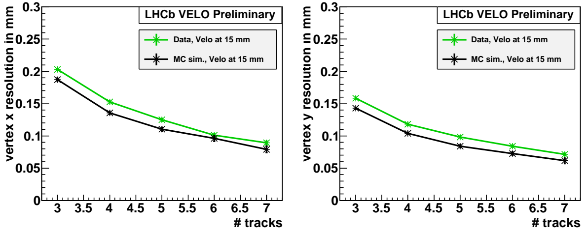
Figure 2: Preliminary estimate of the VELO vertex resolution in the 2009 runs. The resolution in the transverse directions (x and y) for beam-beam interactions are shown as function of the number of tracks per reconstructed vertex.
