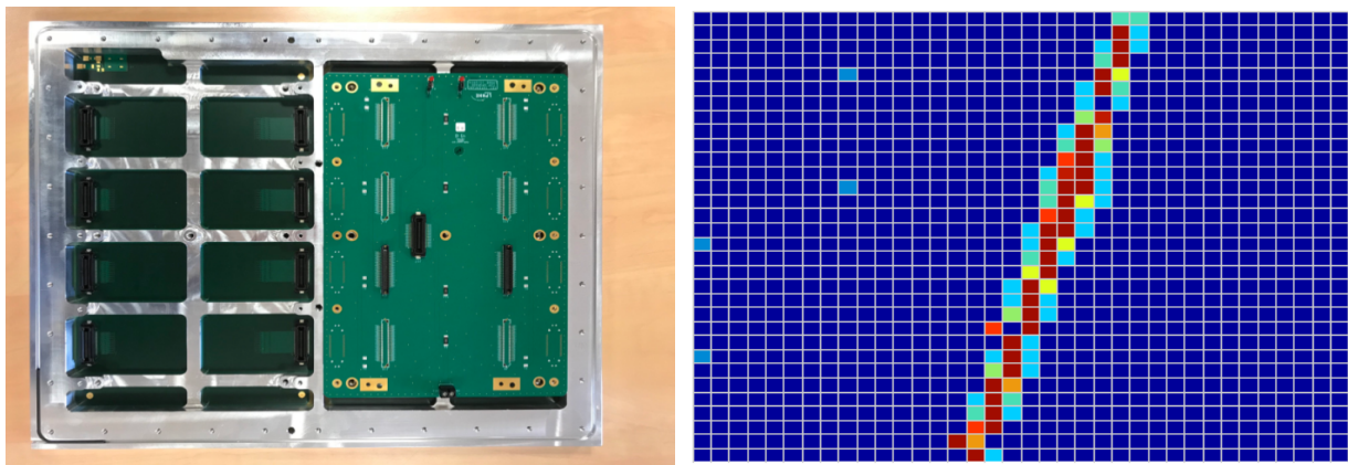
Figure 23: One FEC-mockup board mounted on the MicroMegas prototype detector (left). A cosmic ray track observed with this setup (right).
