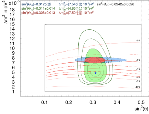
Figure 13: Allowed neutrino oscillation parameter region from all the solar neutrino experiments (green), reactor neutrino from KamLAND (blue) and combined (red).
