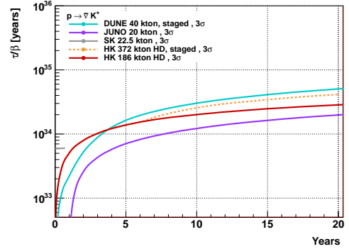
Figure 9: Comparison of the 3\sigma p \rightarrow \bar{\nu}K^+ discovery potential as a function of year for the Hyper-K as well as that of the 40 kton DUNE detector (cyan solid) based on [18] and the 20 kton JUNO detector based on [19]. The red line denotes a single Hyper-K tank, while the orange line shows the expectation when a second tank comes online after six years. The expected discovery potential for Super-K by 2026 assuming 23 years of data is also shown.
