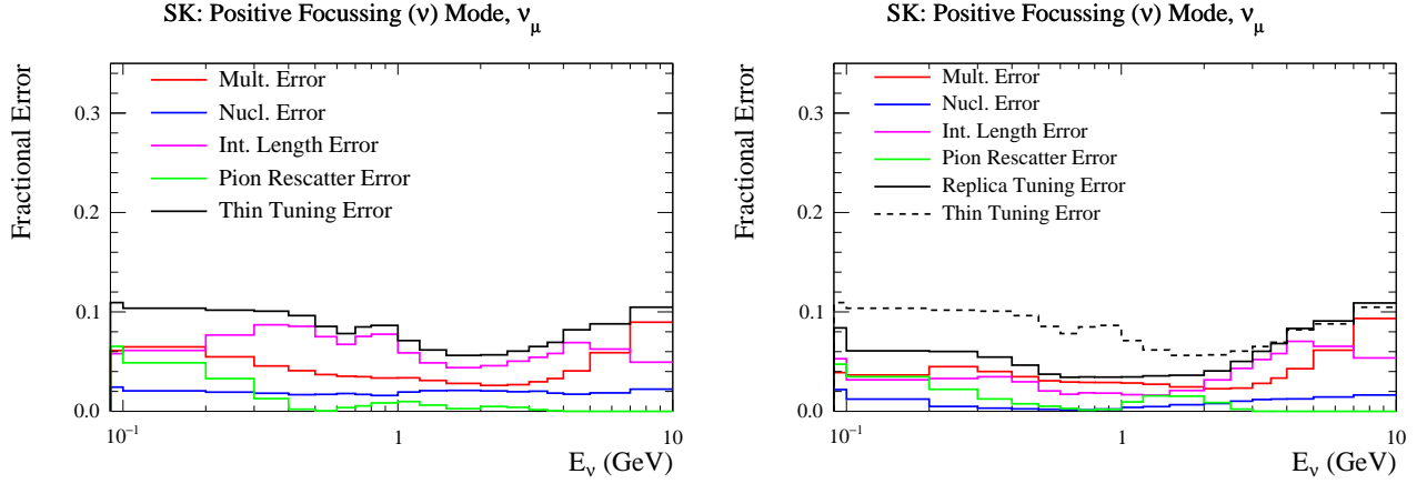
Figure 26: The hadron interaction model uncertainties evaluated on the SK flux prediction. The uncertainties have been calculated for the flux constrained with either purely NA61/SHINE 2009 thin-target data [22] (left side), or using a combination of NA61/SHINE 2009 thin-target and replica-target data [34] (right side, denoted as the replica tuning error). Additional improvement is expected with the NA61/SHINE 2010 replica-target data [35, 33], in particular, the uncertainty in high neutrino energy region because of significant improvement of the knowledge of the kaon yield from the replica target data.
