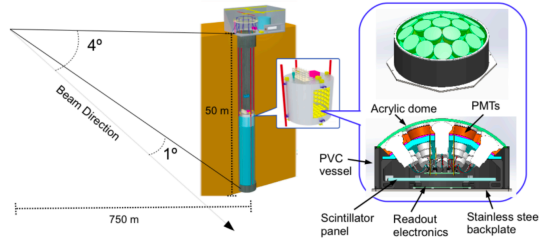
Figure 2: Schematic overview of the IWCD detector.
