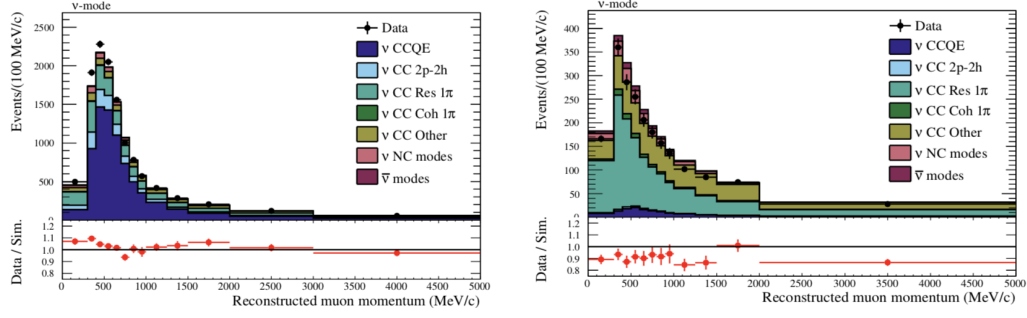
Figure 15: Muon momentum distribution for \nu_\mu CC- 0\pi^+ (left) and CC- 1\pi^+ (right) samples at ND280.
