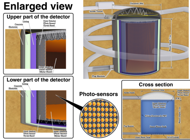
Figure 1: The HK detector
