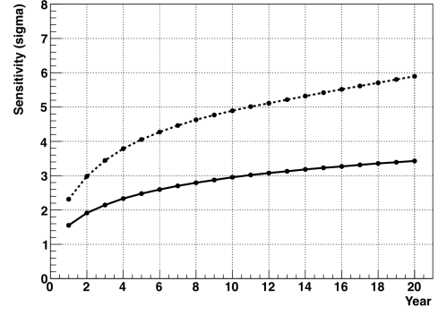
Figure 14: Spectrum upturn discovery sensitivity as a function of observation time. The solid line shows that the energy threshold is 4.5 MeV, while the dotted line shows the 3.5 MeV.
