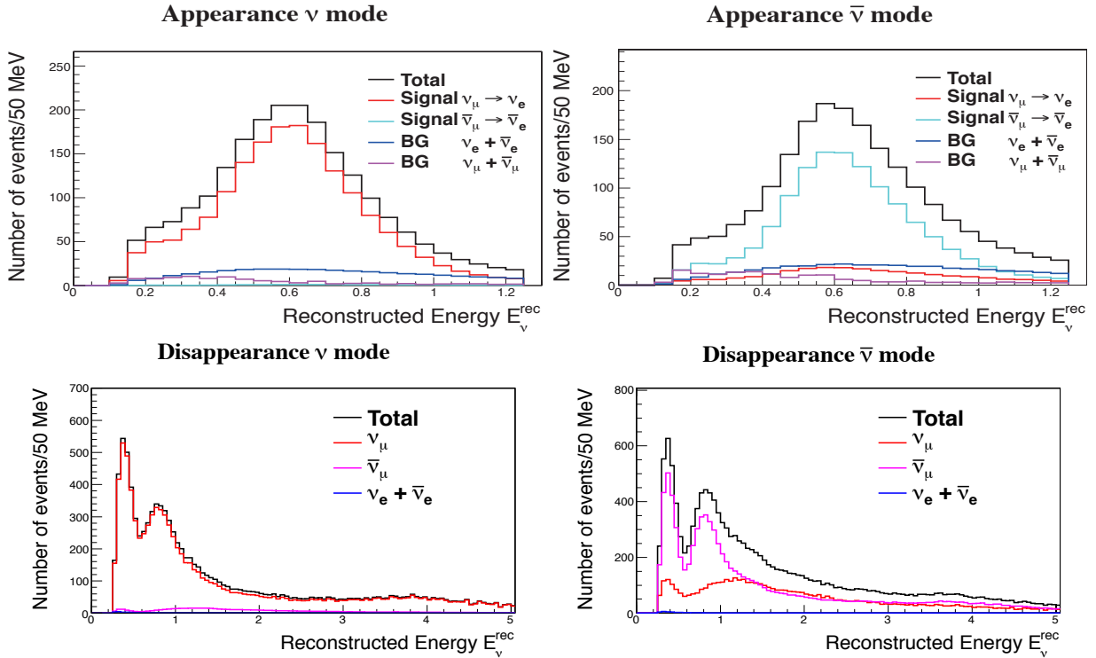
Figure 2: Reconstructed neutrino energy distribution of the \nu_e (top) and \nu_\mu (bottom) candidate events in neutrino beam mode (left) and antineutrino beam mode (right) for 2.7 \times 10^{22} protons on target.
