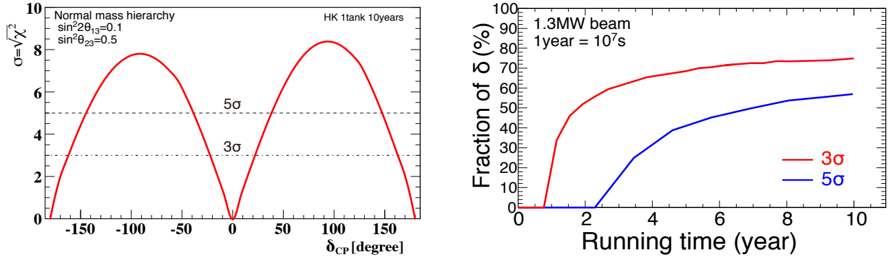
Figure 3: Left : expected significance to exclude \sin \delta_{CP} = 0 plotted as a function of true \delta_{CP} . Right : fraction of \delta_{CP} for which \sin \delta_{CP} = 0 can be excluded with more than 3\sigma (red) and 5\sigma (blue) significance as a function of the running time.
