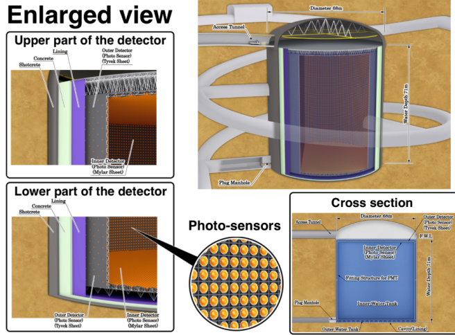
Figure 1: The HK detector
