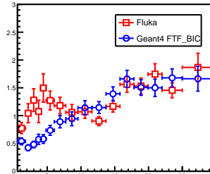
20 < \theta < 40 mrad
