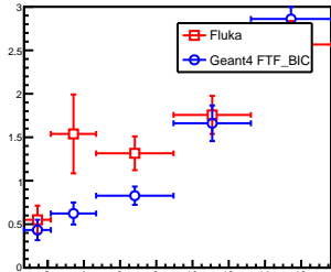
0 < \theta < 20 mrad
