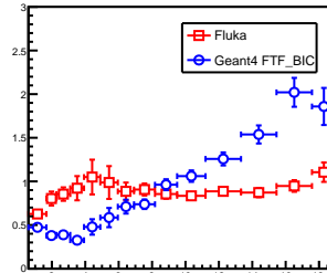
40 < \theta < 60 mrad
