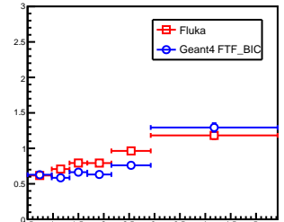
220 < \theta < 260 mrad
