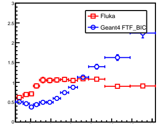
60 < \theta < 100 mrad
