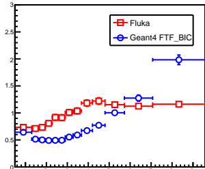
100 < \theta < 140 mrad
