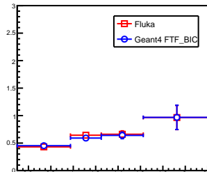
300 < \theta < 380 mrad
