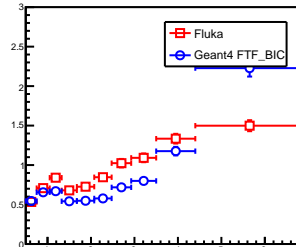
180 < \theta < 220 mrad
