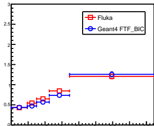
260 < \theta < 300 mrad
