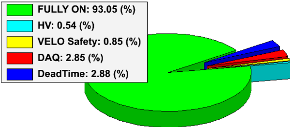
LHCb Efficiency breakdown pp collisions 2010-2012
