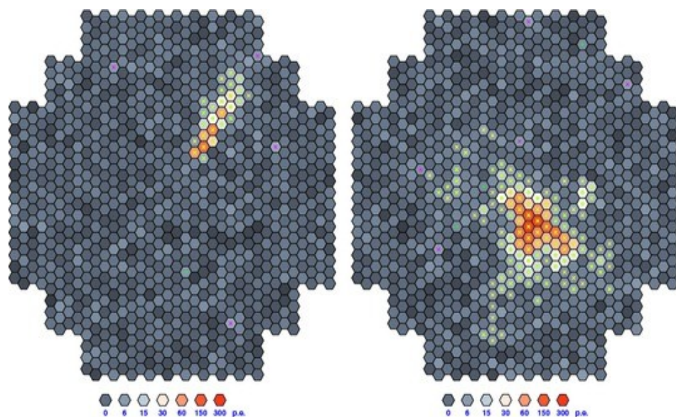
1.0 TeV gamma shower
