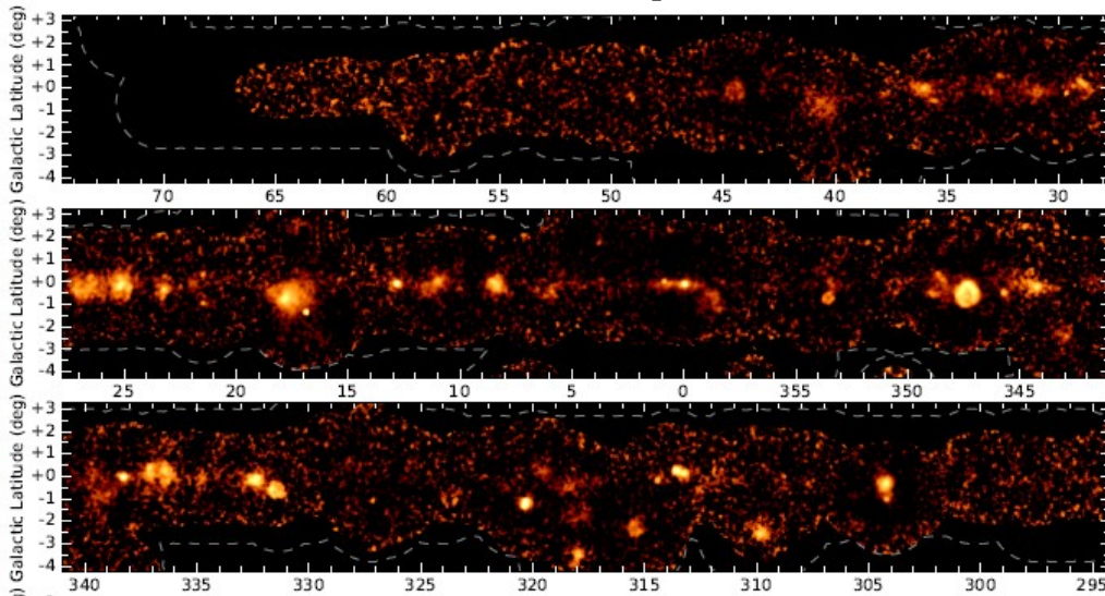
Real data (HESS GPS), 4 Telescopes
