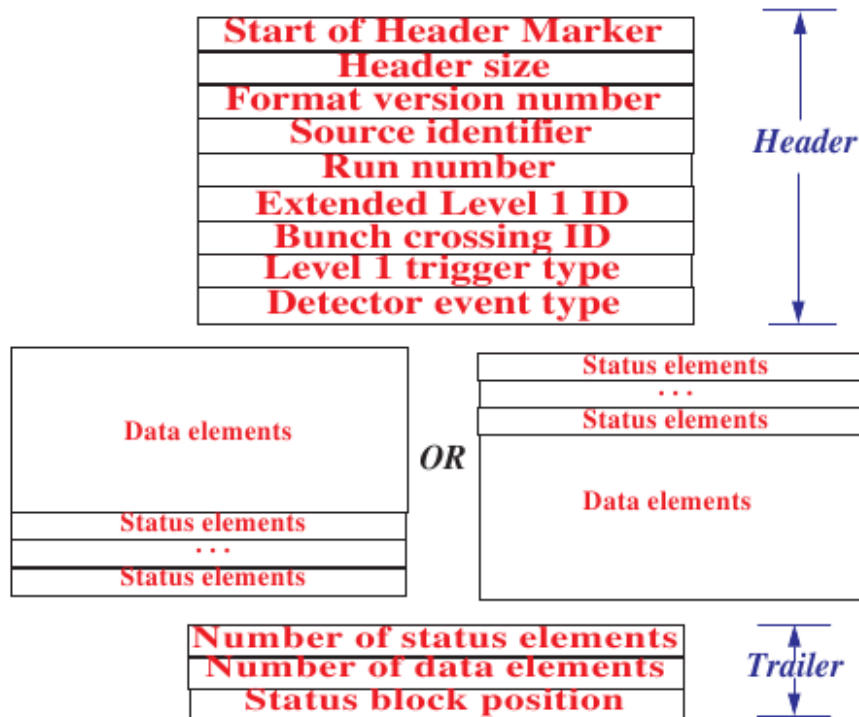
Figure 3: The ROD fragment format.
