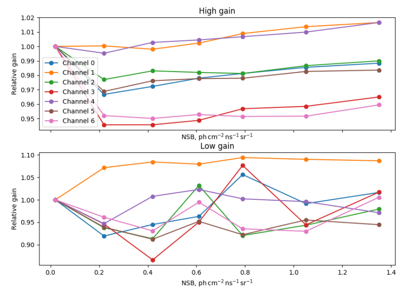
Gain variation with NSB (Channels 70-76)
