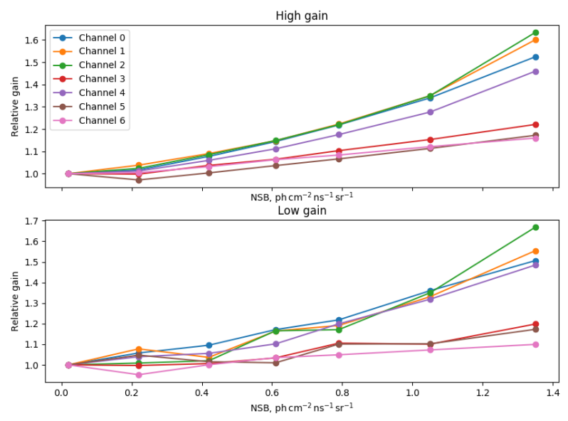
Gain variation with NSB (Channels 0-6)
