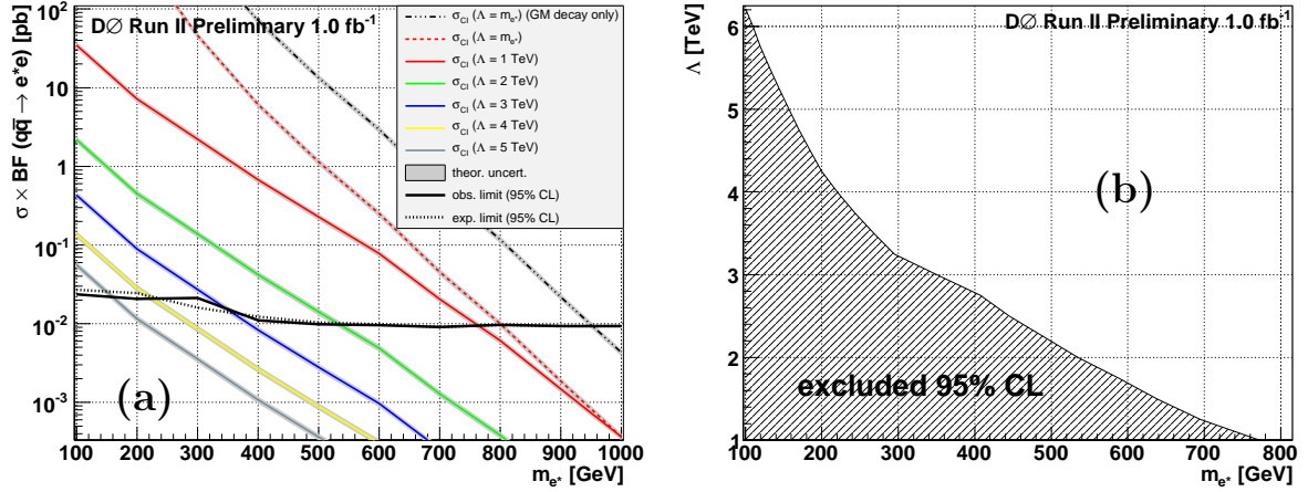
Figure 5: Limits on excited electrons from D0. (a) shows the limit on the cross-section times branching ratio as a function of the mass of the excited electron. (b) shows the limit on the compositeness scale vs. the mass of the excited electron.
