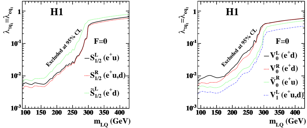
Figure 6: Limits on the coupling constants \lambda_{\tau q_1} = \lambda_{eq_1} as a function of the leptoquark mass m_{LQ} for F=0 scalar (left) and vector (right) leptoquarks. Regions above the lines are excluded at 95% CL. The notation q_1 indicates that only processes involving first generation quarks are considered.
