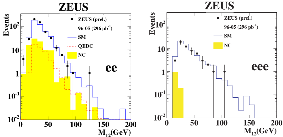
Figure 3: Comparison of the distribution of the invariant mass M_{12} of the two highest P_T electrons in the ZEUS multi-electron search to the SM expectation. The comparison is shown for the ee (left) and eee (right) topologies.
