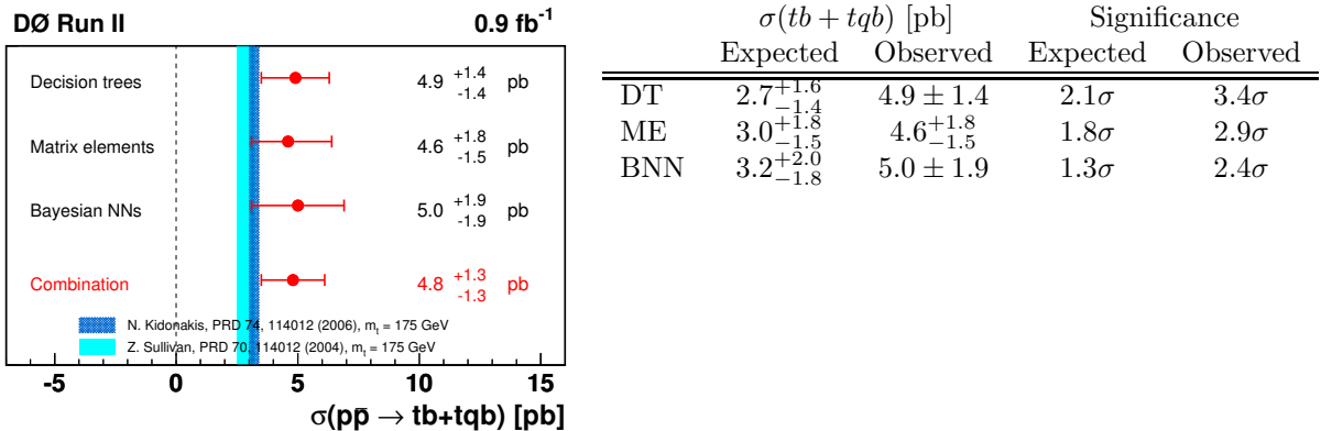
Figure 3: The observed results including the combination (left); and the expected and observed cross sections and significance for the three different multivariate analyses (right).
