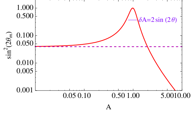
FIG. 7: The effective mixing angle in matter vs. the “matter to vacuum strength parameter” A (red, solid) compared with the vacuum mixing angle (purple, dashed). Here \theta = 0.1 is assumed, which also regulates the width of the peak of the solid curve, as shown.
