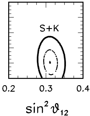
Solar &amp; KamLAND
