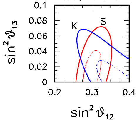
Solar, KamLAND
