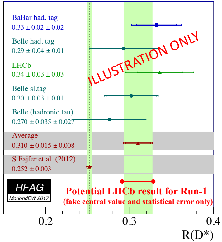
Figure 2 – Potential LHCb statistical uncertainty with Run 1 data, compared to previous measurements of \mathcal{R}(D^*) , the World Average and the SM prediction.
