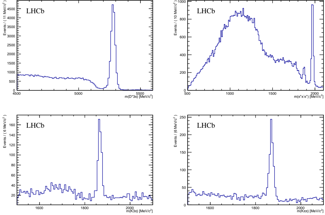
Figure 1 – (top left) D^*3\pi invariant mass distribution for normalization events. (top right) \pi^+\pi^-\pi^+ invariant mass distribution; the peak in the D_s^+ region is used to extract the B \rightarrow D^*D_s^+X control sample. (bottom left) K^-\pi^+\pi^-\pi^+ invariant mass distribution; the peak in the D^0 region is used to obtain the B \rightarrow D^*D^0X control sample. (bottom right) \pi^+\pi^-\pi^+ invariant mass distribution with kaon hypothesis on the \pi^- ; the peak in the D^+ region is needed to build the B \rightarrow D^*D^+X control sample.
