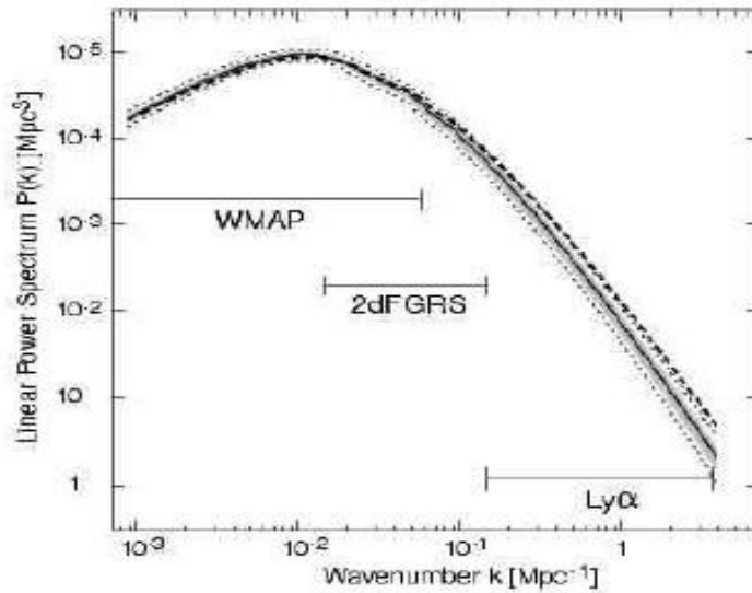
Figure 2. The power spectrum as obtained from WMAP measurements of the CMB spectrum, together with the 2dF Galaxy Redshift Survey and Lyman \alpha measurements.
