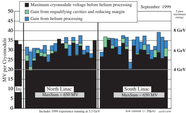
Figure 3. Peak capability of the CEBAF cryomodules.
