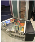
Cray (1980) Centralized
