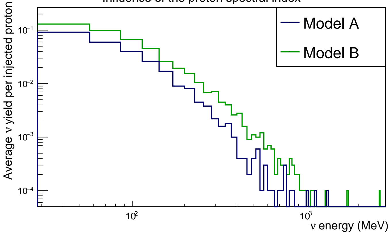
Influence of the proton spectral index
