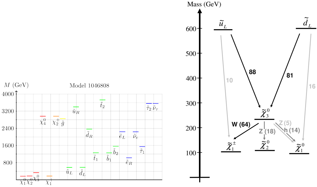
Figure 1 – (Left) Sample seed model spectrum and (Right) the corresponding squark to bino to Higgsino decay pattern.
