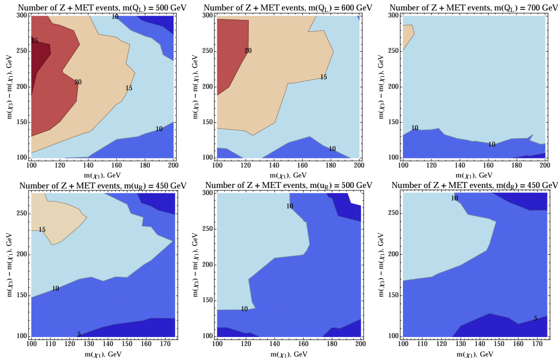
Figure 2 – Signal event rate contours for the ATLAS Z+jets+MET analysis in the bino-Higgsino( \chi_3^0 - \chi_1^0 ) mass difference and LSP( \chi_1^0 ) mass plane. The top three panels correspond to the case of \tilde{Q}_L = 500, 600, 700 GeV from left to right, while the bottom panels are for \tilde{u}_R = 450, 500 GeV and \tilde{d}_R = 450 GeV, left to right.
