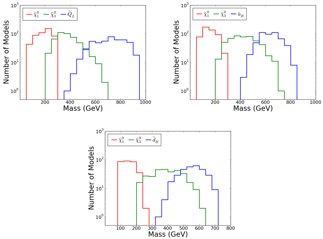
Figure 4 – Mass distributions of the parent squark, \tilde{\chi}_3^0 and \tilde{\chi}_1^0 states for the models from our grid scan that agree with all null search results and yield at least 5 events in the ATLAS Z +MET channel. The top-left, top-right, and bottom panels correspond to the parent squark cases of \tilde{Q}_L , \tilde{u}_R , and \tilde{d}_R , respectively.
