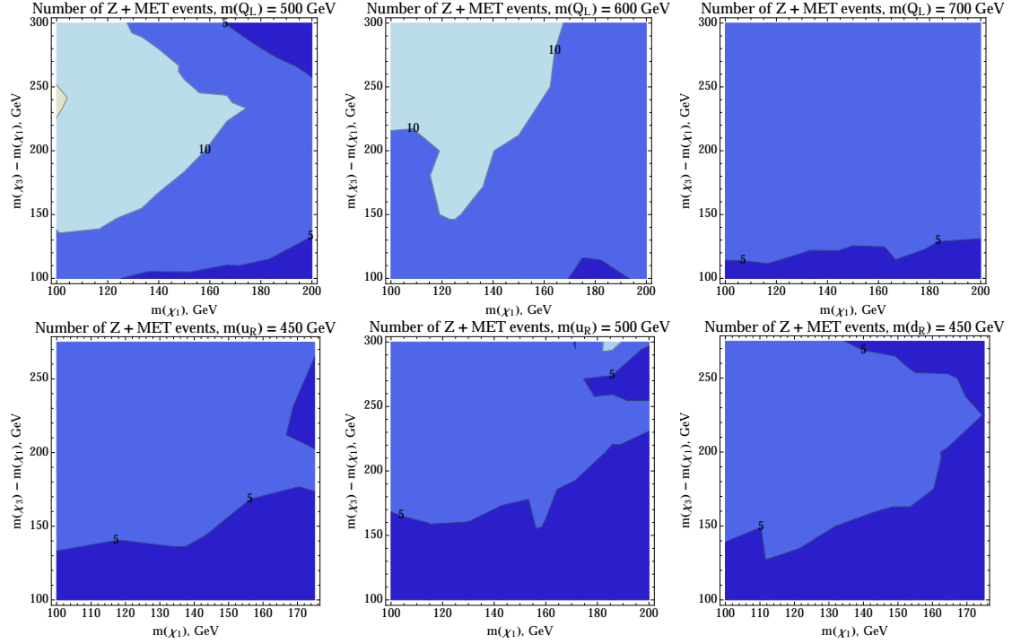
Figure 5 – Same as Fig.2 but now for the ATLAS 13 TeV analysis. For than 10(5) signal events are to be expected in the lightest(darker) region while points in the darkest regions lead to fewer than 5 events.
