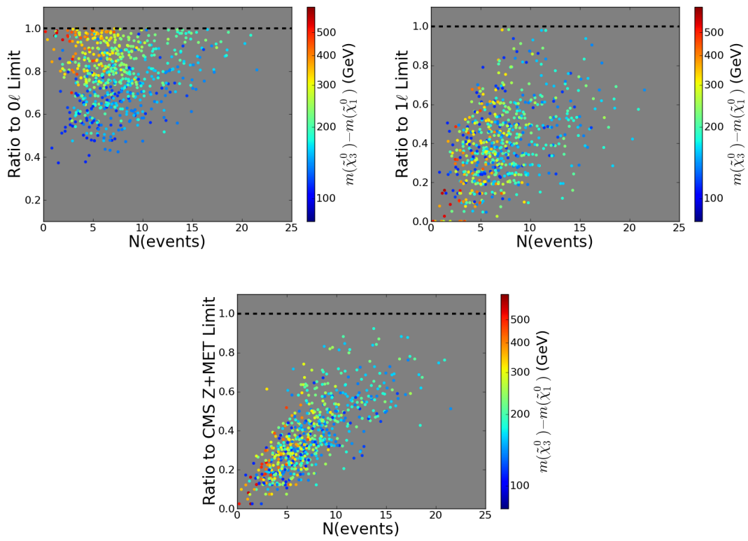
Figure 3 – Ratio of the predicted number of events for the \tilde{Q}_L models in our simplified grid scan to the ATLAS 95% CL search limit for the 0l +jets and 1l +jets channels as well as that for the CMS dilepton search, respectively, as functions of the number of predicted signal events for the ATLAS Z+jets+MET search. The color code corresponds to the value of the \chi_3^0 - \chi_1^0 mass splitting.
