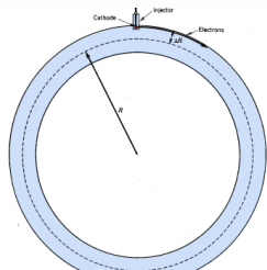
Figure 11.4 Superior geometry for the current betatron.
